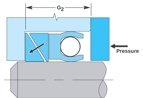
Gland width for standard OmniSeals plus back-up ring
