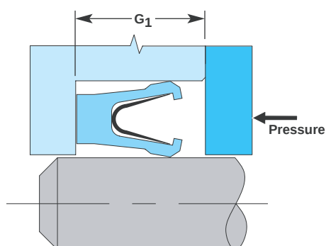
Gland width for extended heel OmniSeals
