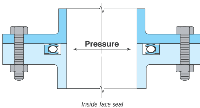
Static Face Seal (Internal Pressure)
