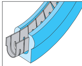
OmniSeal RACO 1100A Spring Design
