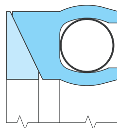
High pressure seals with back-up rings
