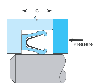
Gland width for standard OmniSeals
