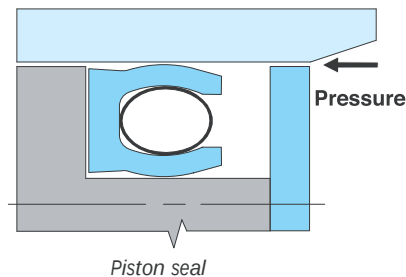
Piston seal
