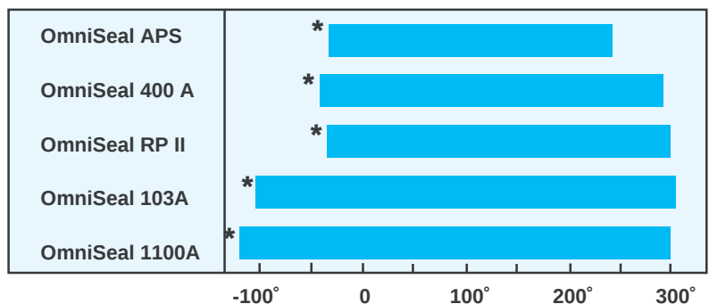
Seal Design Vs. Temp. Chart.
